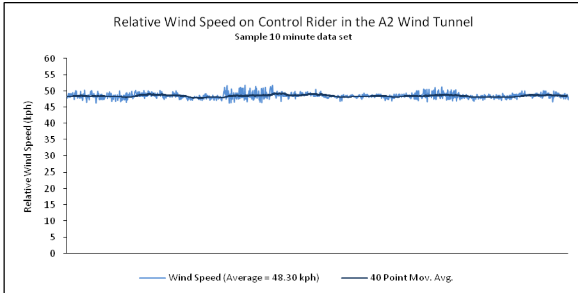
Figure 3: Relative wind speed in the wind tunnel, set to 48.3 kph (30 mph)
