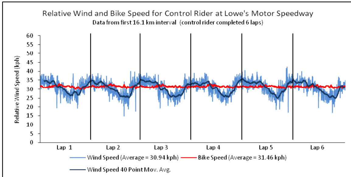
Figure 4: Relative wind and bike speed for the control rider at Lowe's Motor Speedway
