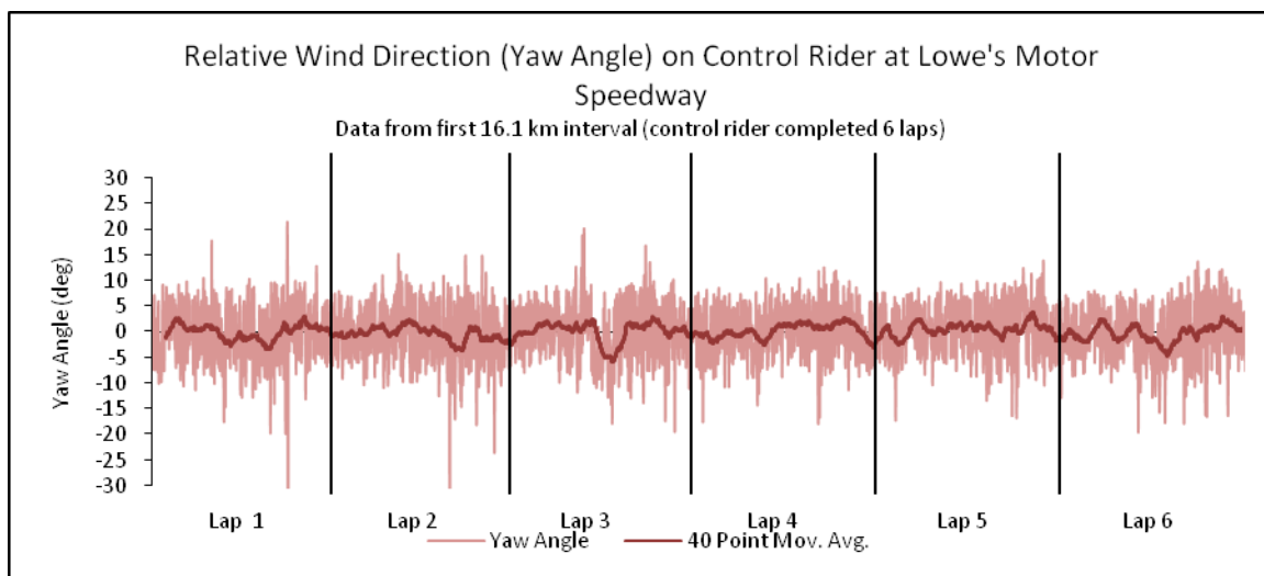
Figure 6: Relative yaw angle experienced by the control rider during the first test interval at Lowe's Motor Speedway
