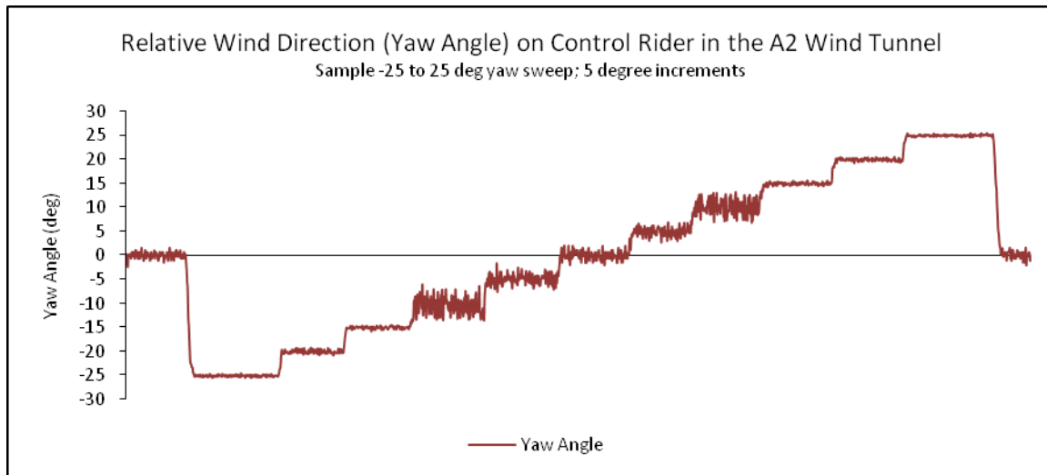
Figure 5: Yaw angles measured with the aerodynamic probe in the wind tunnel; each yaw step represents a 15 second data set
