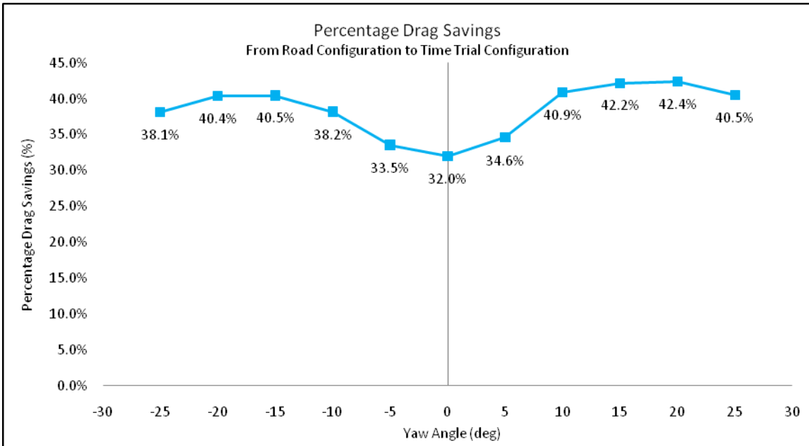
Figure 2: Percentage drag savings from road to time trial configurations
