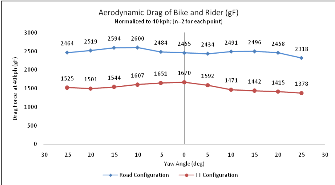
Figure 1: Aerodynamic drag of bike and rider in grams of force (gF), normalized to 40 kph
